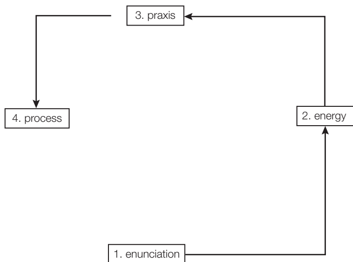
FIGURE 8.8 Enunciative hyper-complexity
