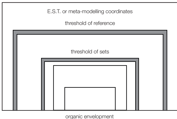
FIGURE 8.6 Chronic discursivity
